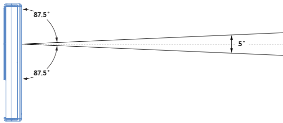
CAL 32, 5-Degree Beam
