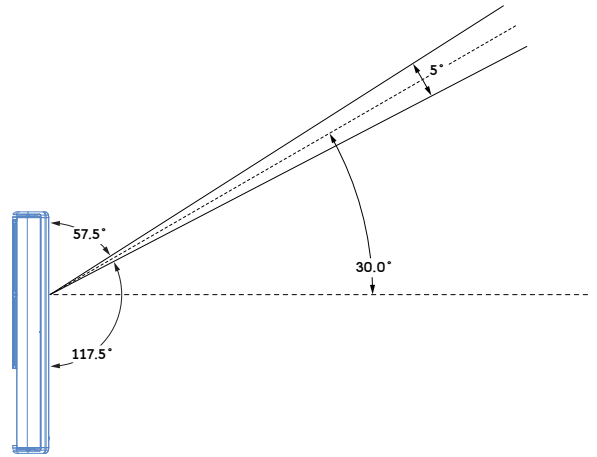
CAL 32, Beam Steered +30 Degrees
