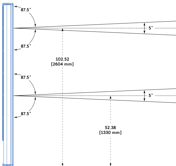
CAL 96, Top Split Beam Coverage
